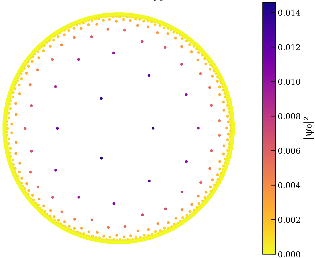
Ground state distribution: Hyperbolic \{3,7\}
